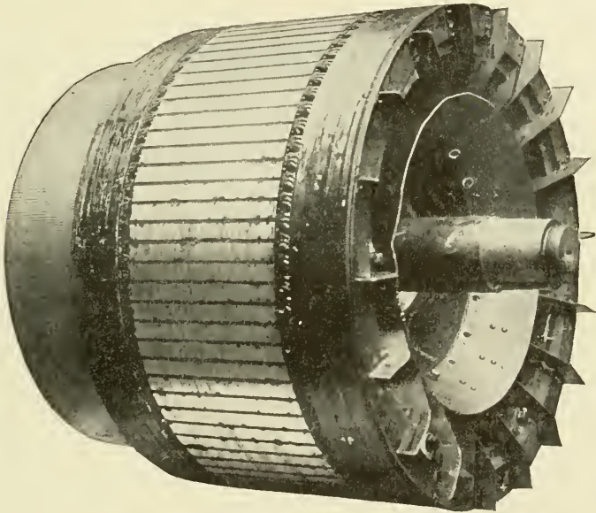
Fig. 263. Armature of Motor Shown in Fig. 261
